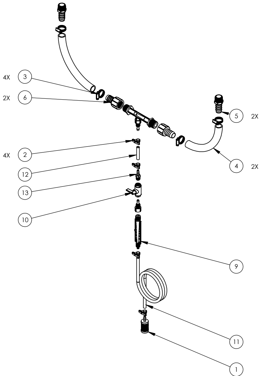
(EXPLODED VIEW) (FOR REFERENCE ONLY)
