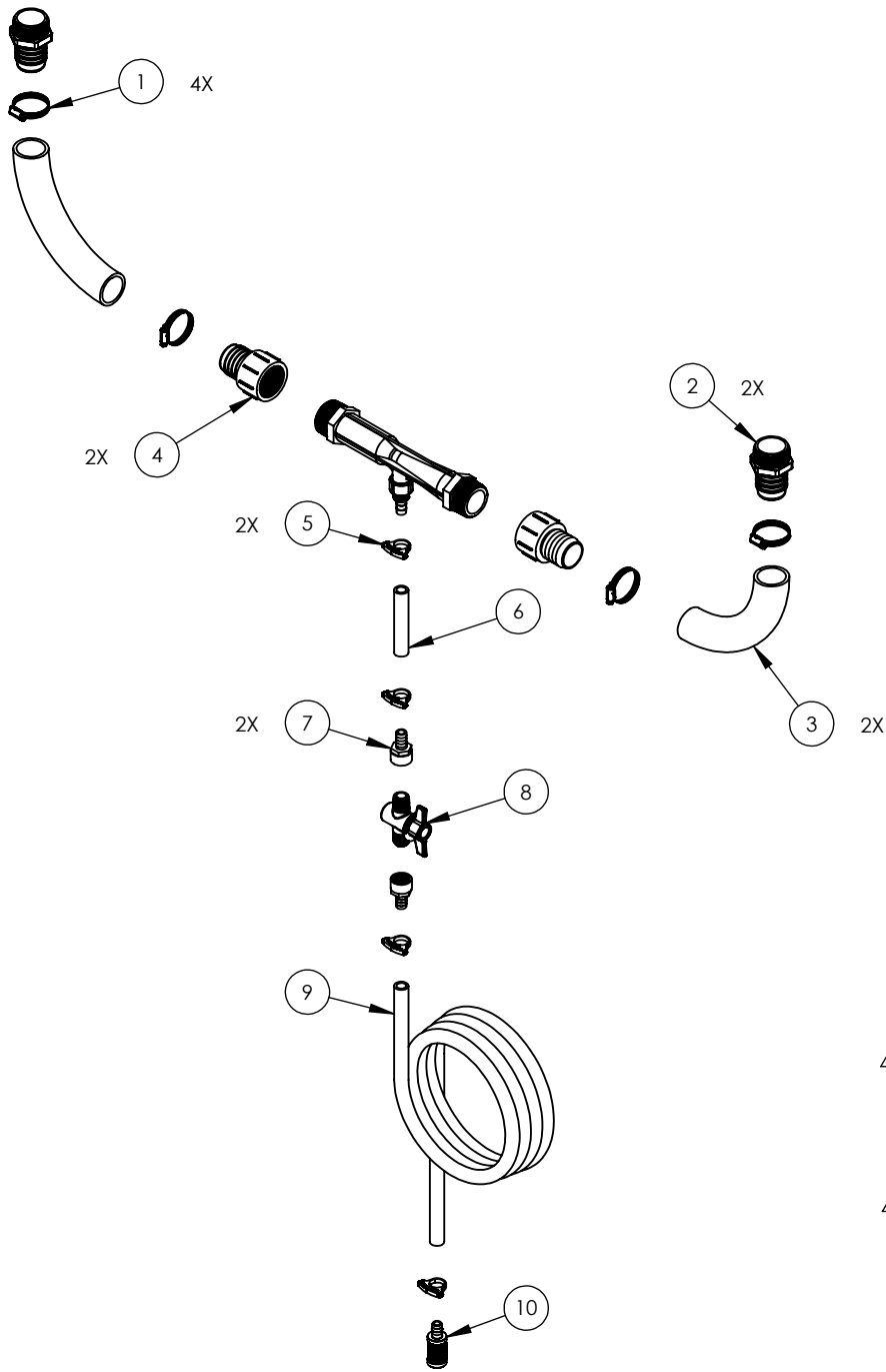
(EXPLODED VIEW) (FOR REFERENCE ONLY)
