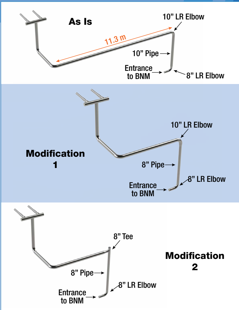
FIGURE 1: Contactor 4-1 SVI-BNM piping options
