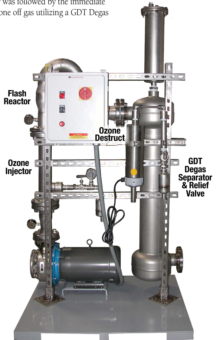
FIGURE 1: GDT process skid
