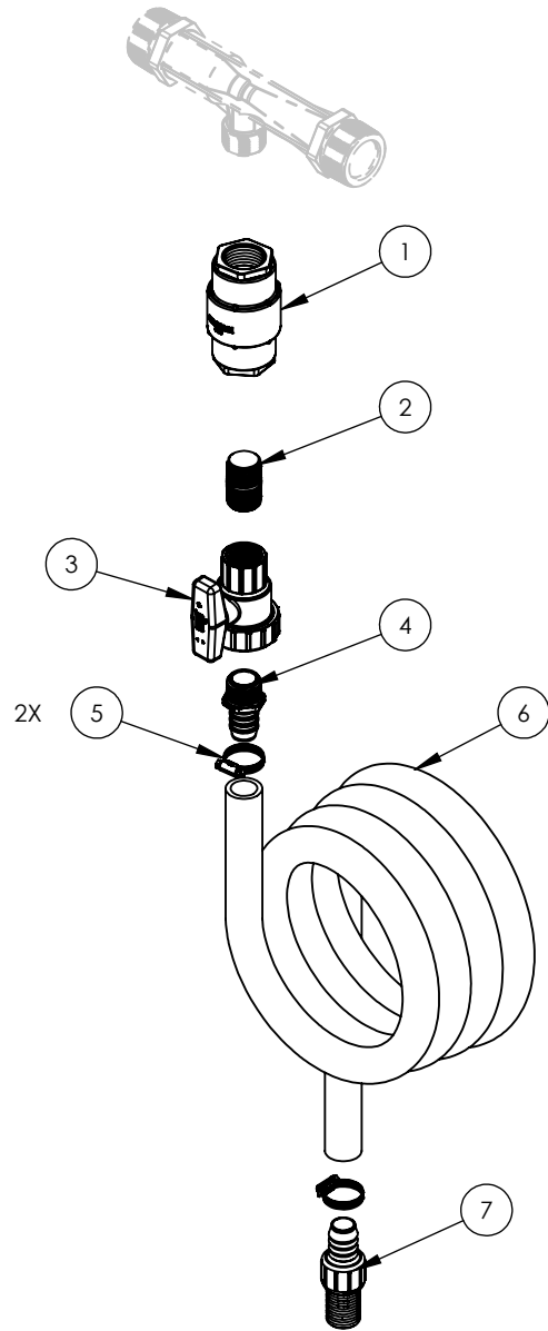
(EXPLODED VIEW) (FOR REFERENCE ONLY)
