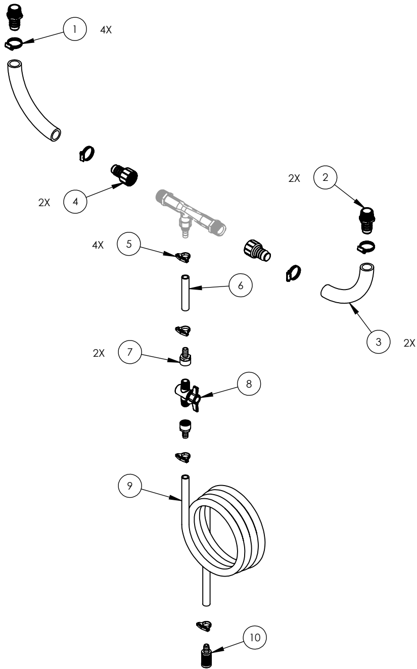
(EXPLODED VIEW) (FOR REFERENCE ONLY)
