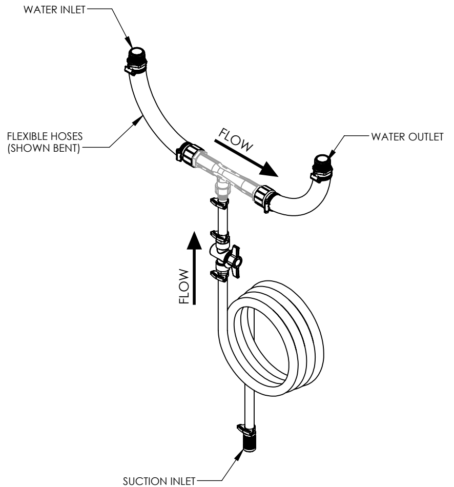
(ISOMETRIC VIEW) (FOR REFERENCE ONLY)
